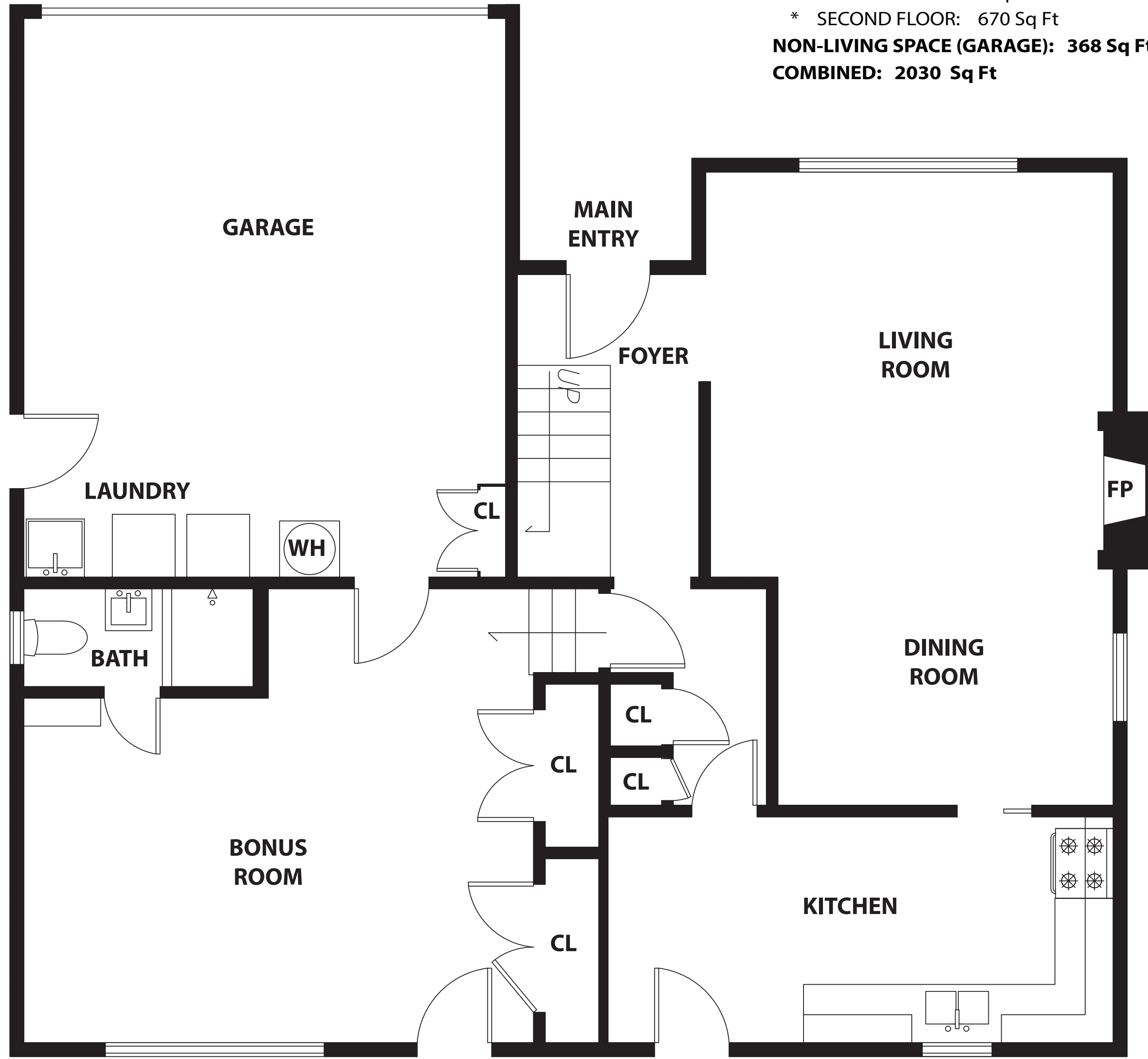
FIRST FLOOR
